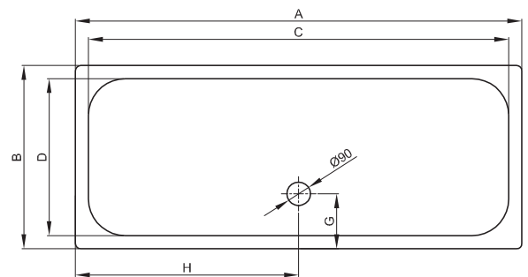
Waste position - A 1600mm and above
