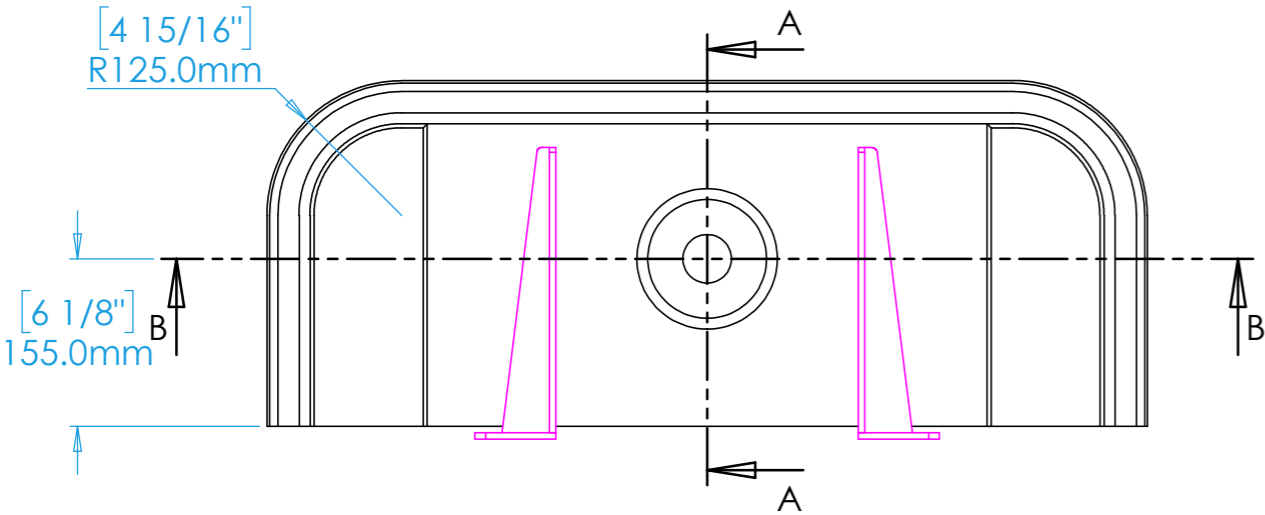
Underside View
